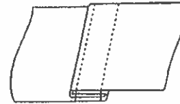
Seam Type LSc-2 (Modified)
